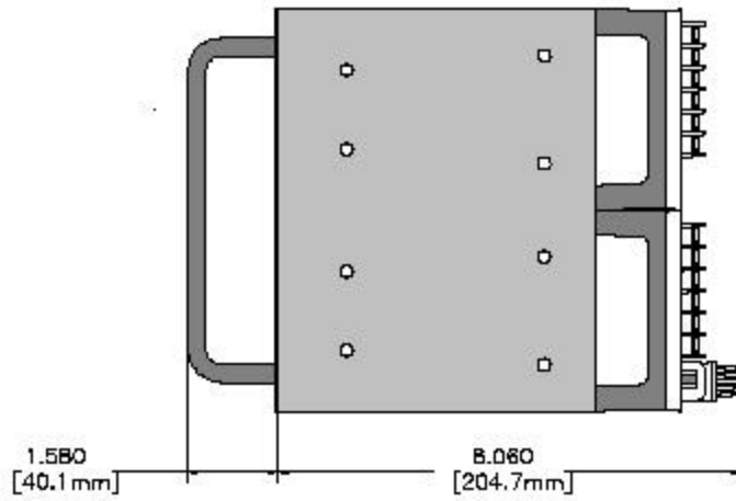
Figure 2-24 Dimensional Information of X11CA RR-4000 (DWG NO. X11C513)
