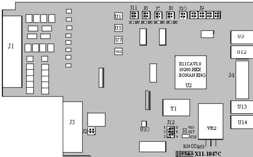
Figure 2-7 X11-1047C Module
