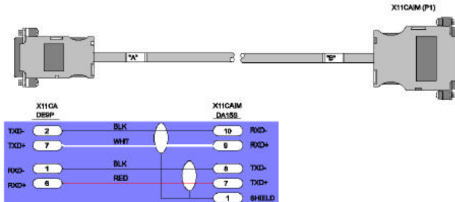
Figure 2-10 Cable for X11CA to X11CA-IM Connection
