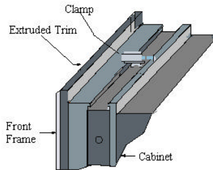
Figure 2-15 Inserting the Clamp into the Top Center of the Cabinet Groove.
