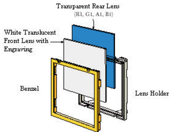
Figure 2-1 Displays and Nameplates
