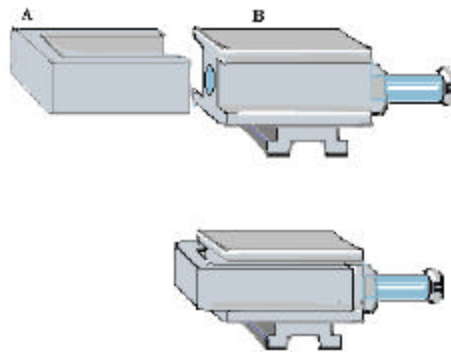
Figure 2-14 Assembling The Clamp Parts
