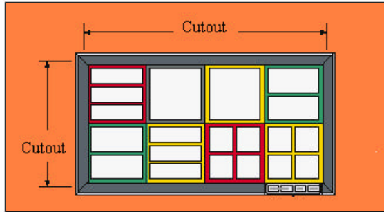
Figure 2-13 The Front View Of The Cabinet After Positioning In The Panel
