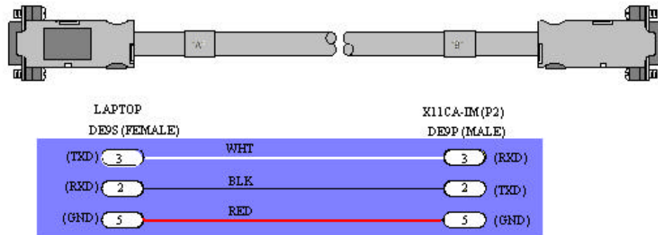
Figure 2-11 RS232 Cable from Host PC to X11CA-IM Connection
