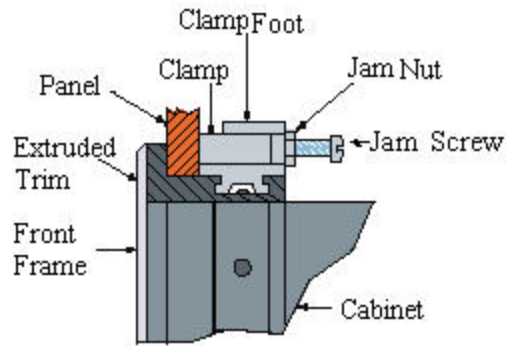
Figure 2-16 Detail A
